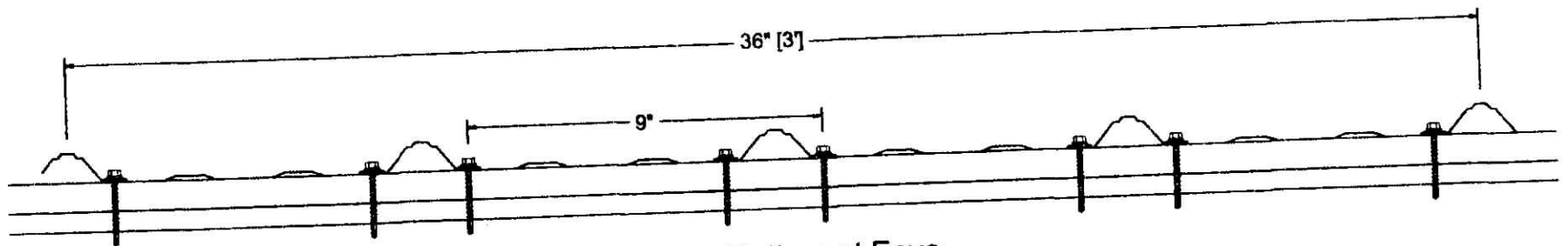
Fastener Pattern at Eave
