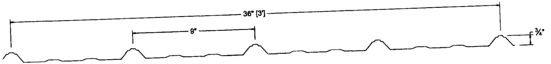
South Rib Profile
